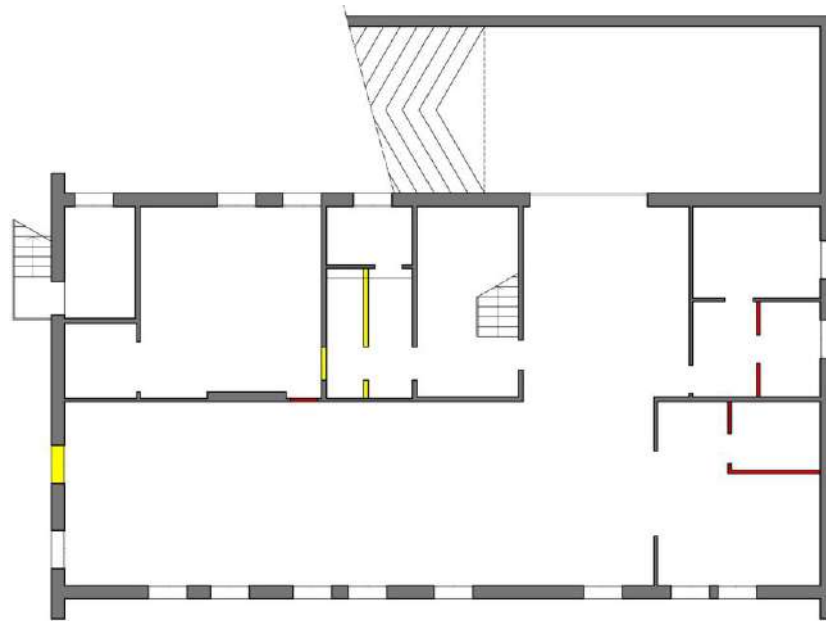
PIANO SEMINTERRATO
