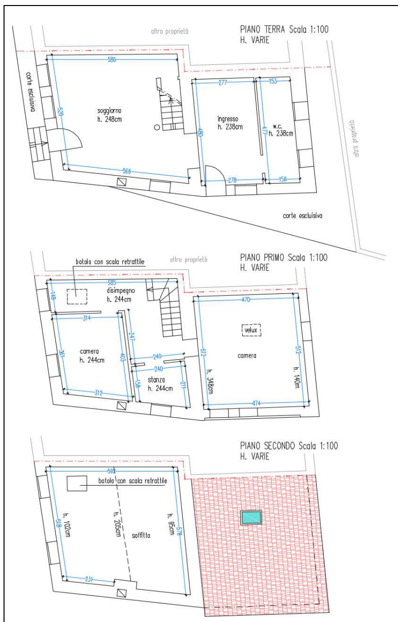
Planimetria immobile – particella 816
