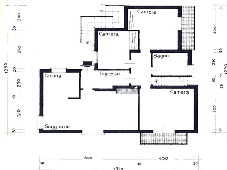
PIANO SEMINTERRATO
